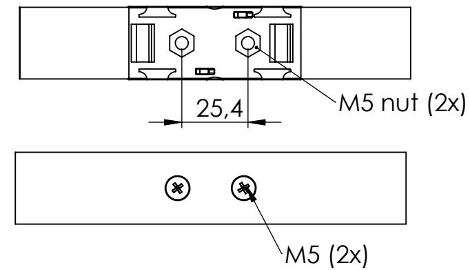
Mounting with Simco bracket small
