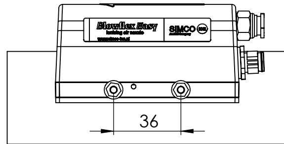
Side mounting
