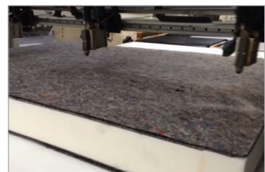
Spray application on fleece
